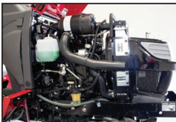
Engine - right side view
